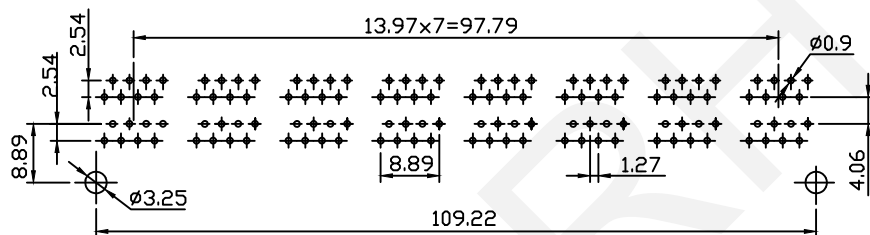
PCB Layout
